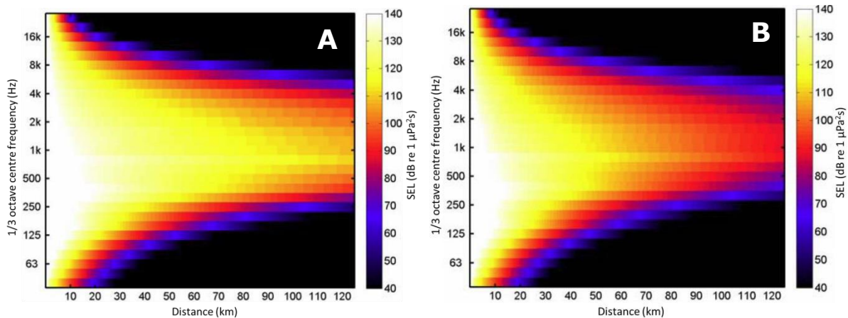
Figure 18. Predicted 1/3 octave band spectrum of the sound exposure level (SEL) at 1-m above the seabed, as a function of distance from Luchterduinen tower 28, during a single pile-drive at an energy level of 1400 kJ: A) with no wind interference; B) with wind at 6-8 m/s, creating noise on the surface that reduces sound propagation. Figure taken from de Jong et al. (2013).
