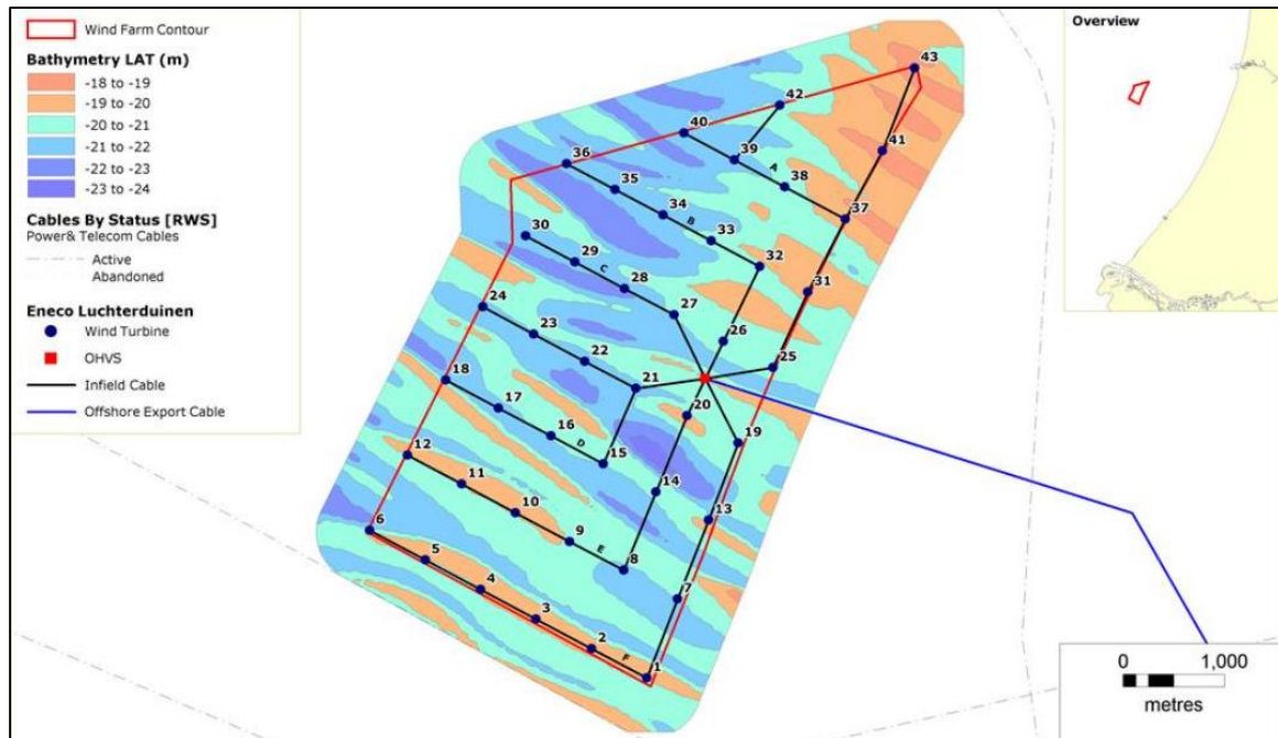
Figure 5. Locations for activities, wind-turbine and cable locations, and bathymetry at Luchterduinen (map supplied by ENECO).
