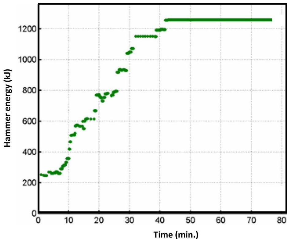
Figure 7. An example of the change in energy level and frequency of blows over time during pile-driving of a turbine tower. This is a scenario based on a total of 2500 hammer blows and a maximum energy of 90% of 1400kJ. Figure adapted from de Jong et al (2013).
